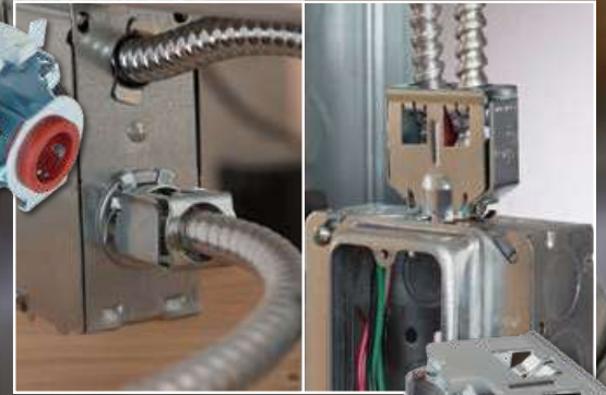
AMC-50QI E-Z LOCK™ CONNECTORS
