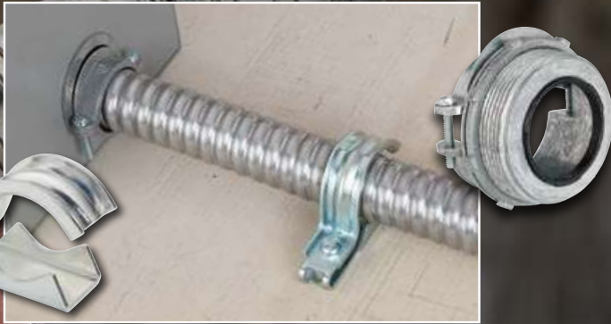
680 SERIES TWO SCREW STRAP CONNECTORS
